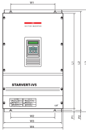
● Dimensions of each capacity (mm[inches])
