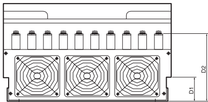
● Dimensions of each capacity (mm[inches])
