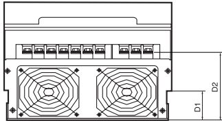
● Dimensions of each capacity (mm[inches])
